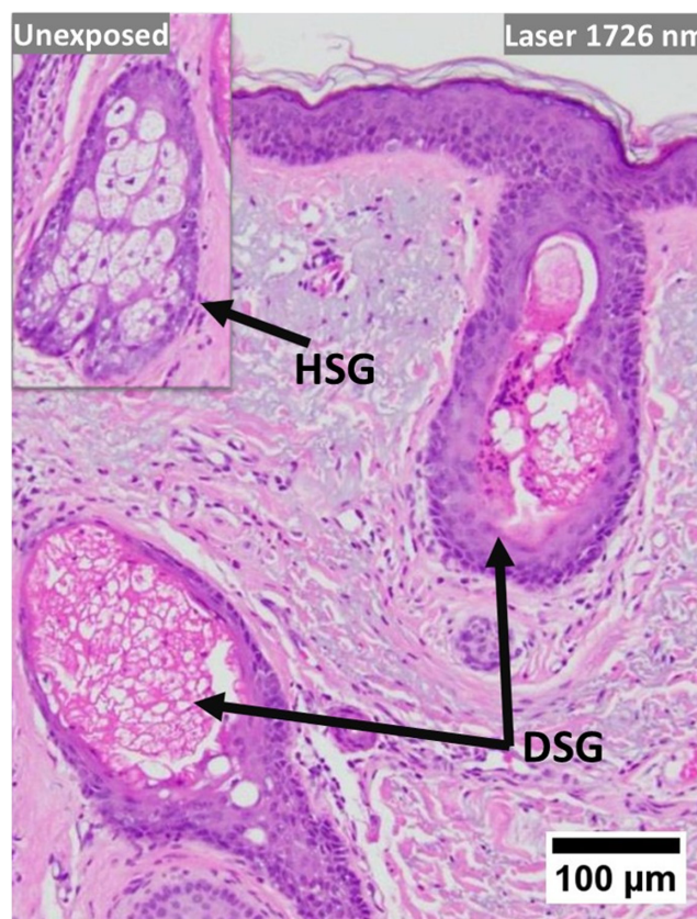
FIGURE 1 Histology image of human skin exposed to 1726 nm. Laser exposure shows selective targeting of sebocytes resulting in damaged sebaceous glands (DSG) preserving the dermis and the epidermis; the inset shows the unexposed skin, preserving healthy sebaceous glands (HSG).
